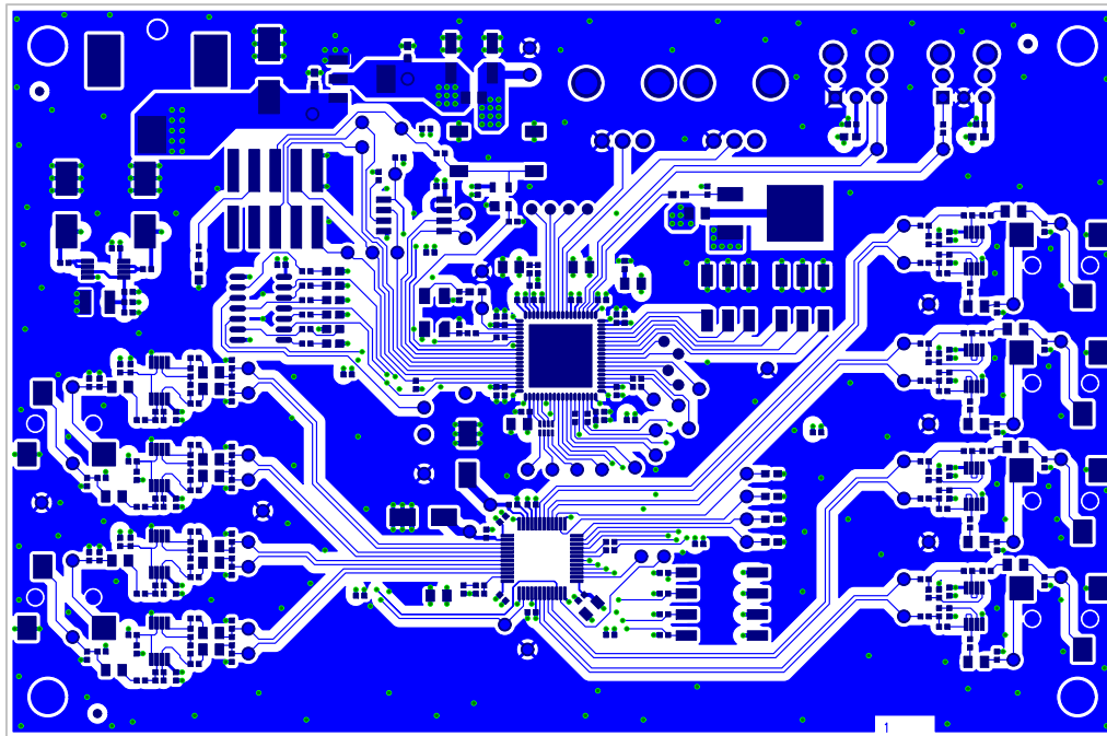
EVAL-ADAU1466Z Rev. B (Primary Side View) Primary Side - Layer 1
