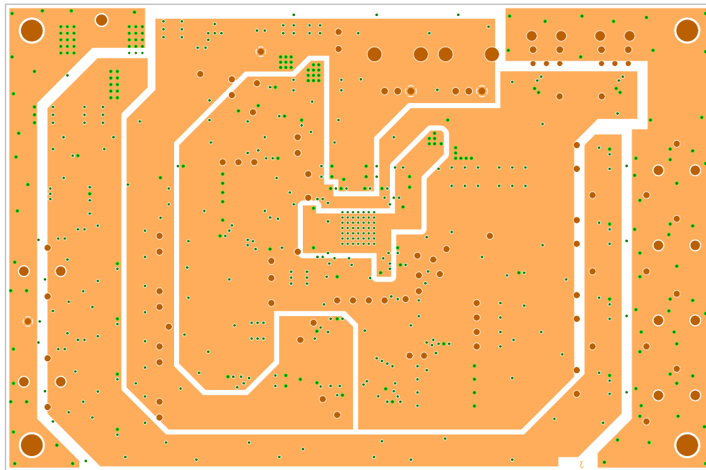
EVAL-ADAU1466Z Rev. B (Primary Side View) Layer 3 Inner 1
