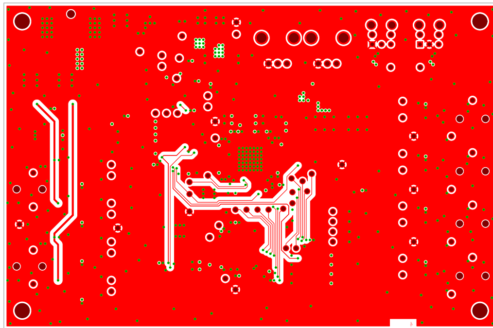
EVAL-ADAU1466Z Rev. B (Primary Side View) Secondary Side - Layer 8
