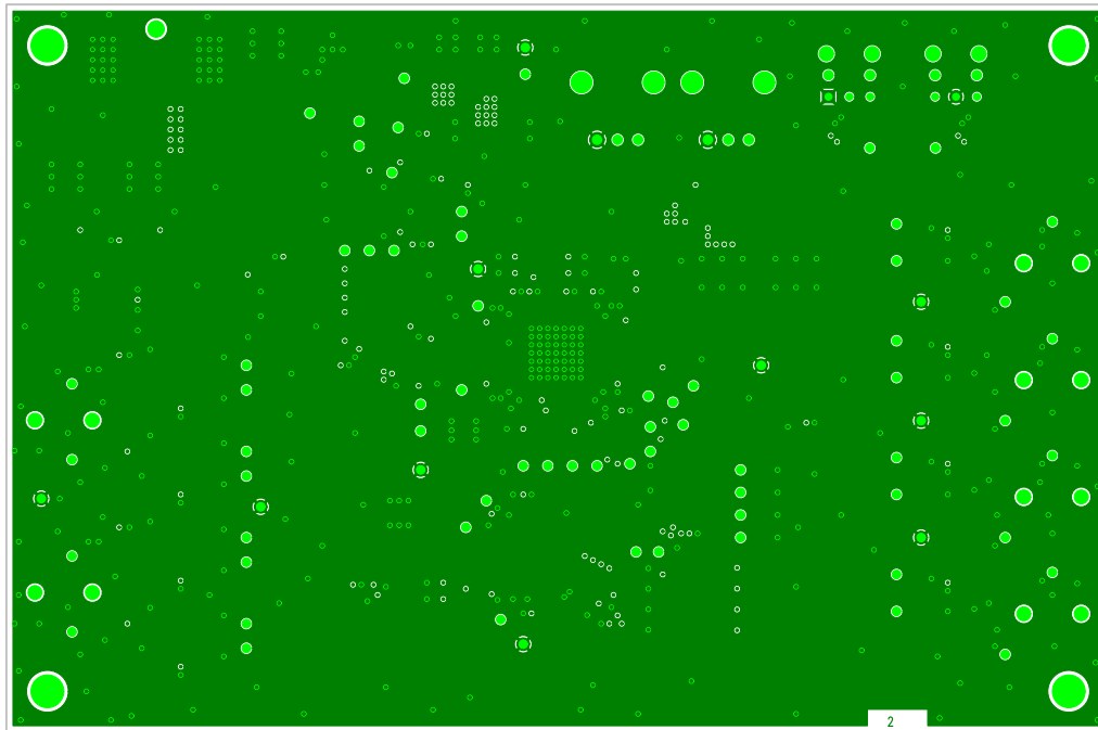
EVAL-ADAU1466Z Rev. B (Primary Side View) Layer 2 GND 1
